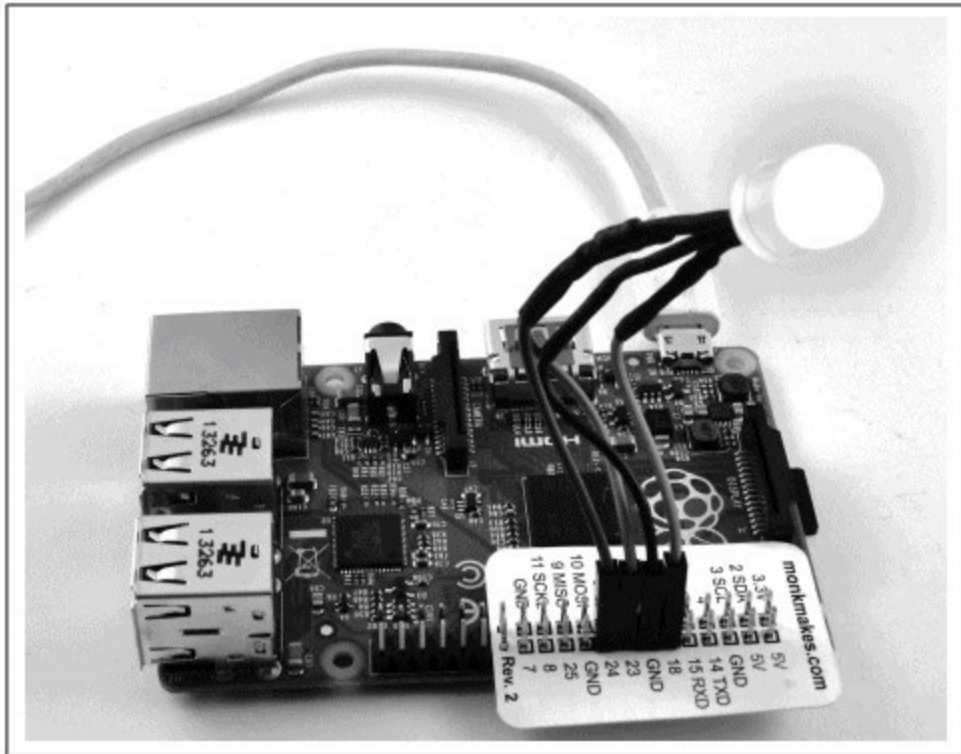
图9-12 Raspberry Squid
