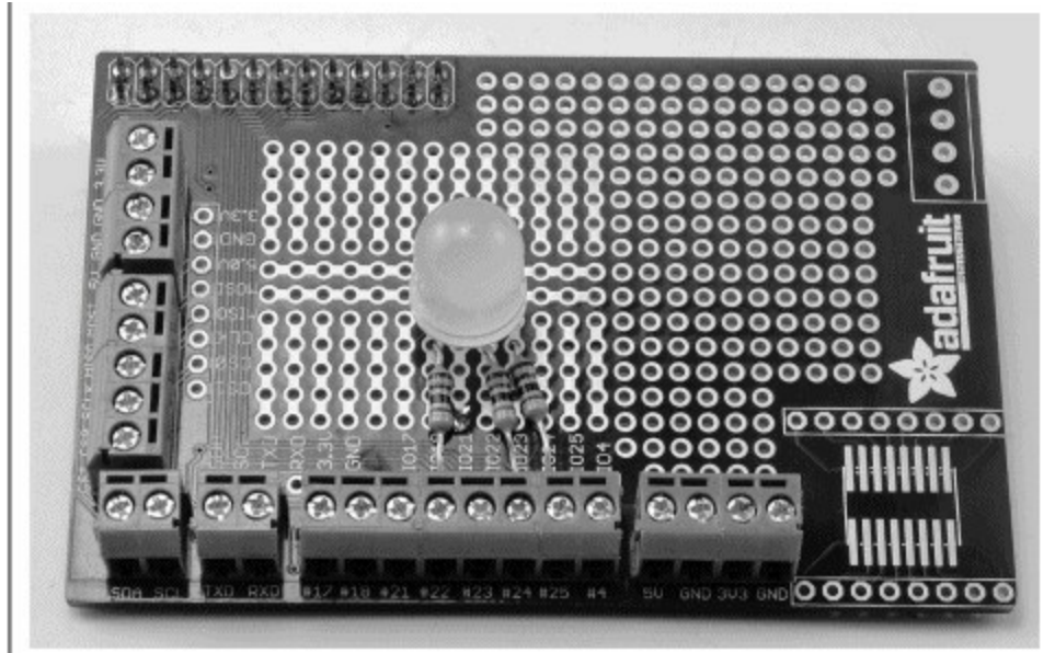
图9-27 Pi Plate上焊接好的RGB LED
