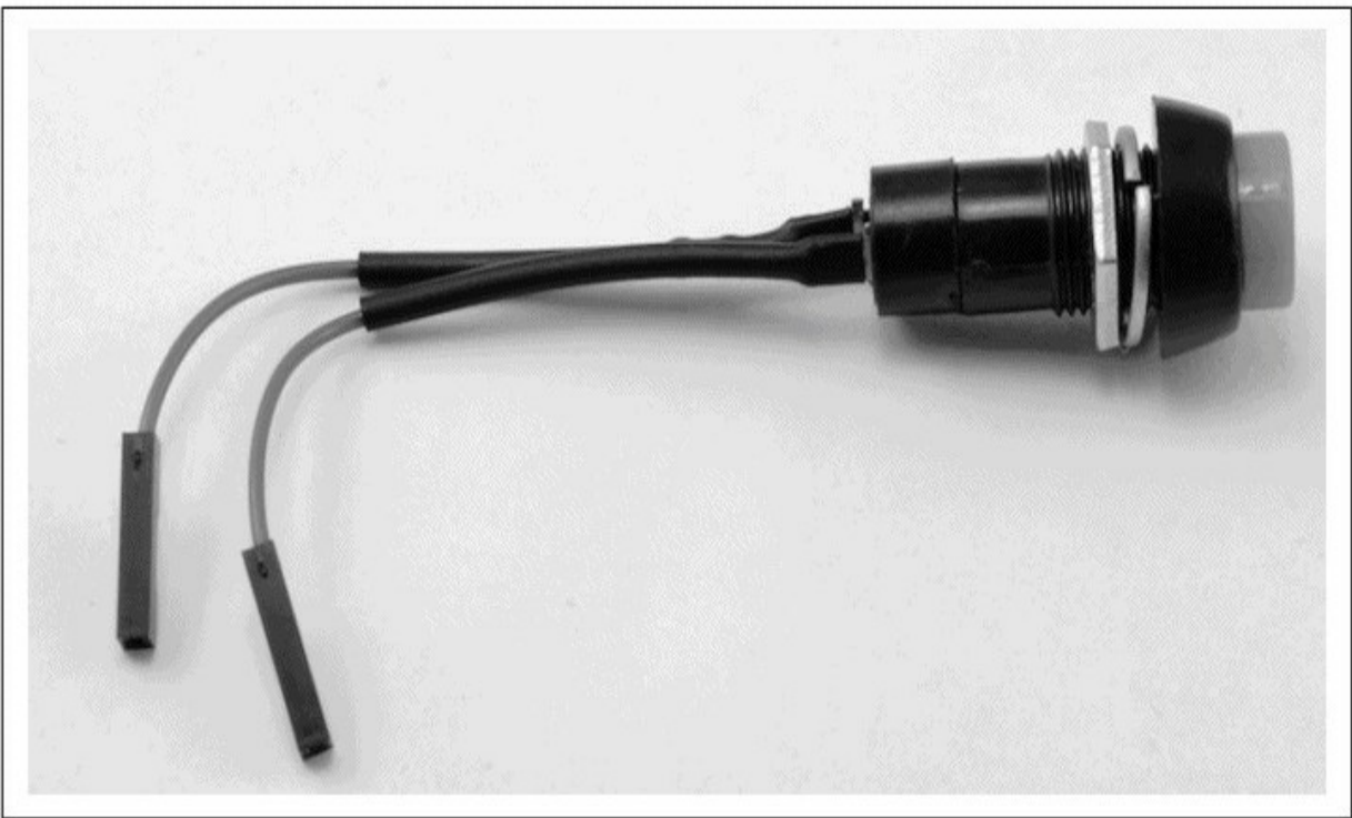
图12-2 Squid Button
