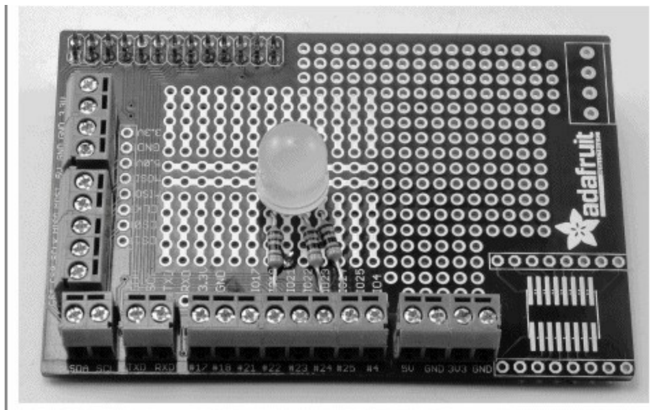
图9-22 Pi Plate
